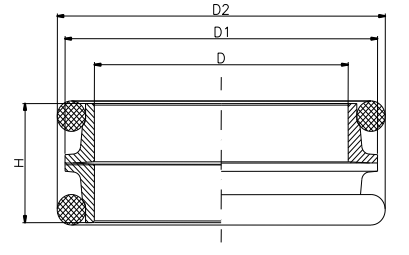
OR-KESİT
