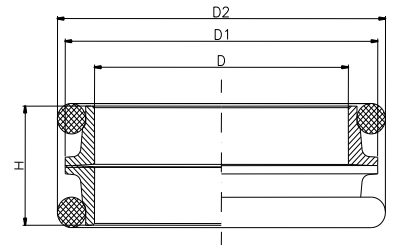
OR-KESİT
