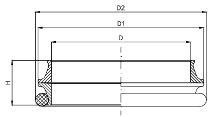
OR-KESİT
