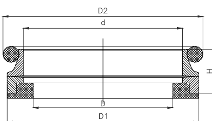
OS-CROSS-SECTION
