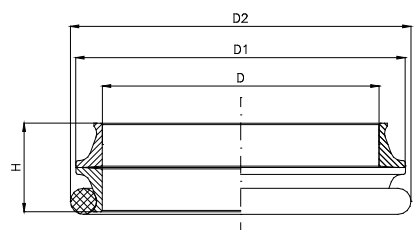
OR-CROSS-SECTION
