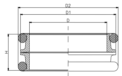
OR-CROSS-SECTION
