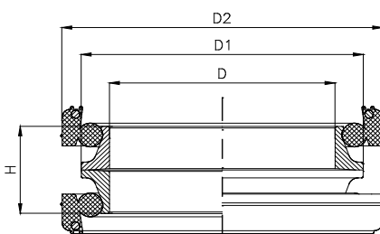
DD-CROSS-SECTION
