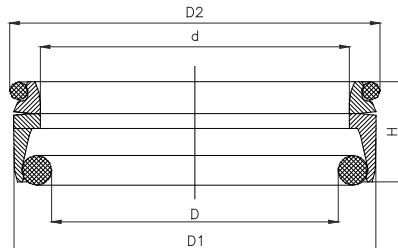
OS-CROSS-SECTION
