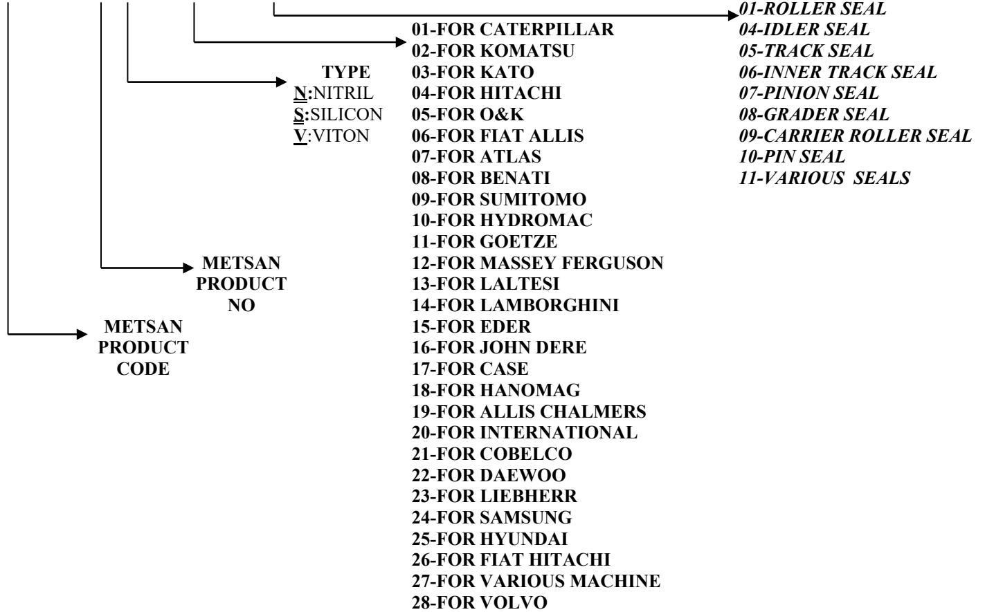
LL-CROSS-SECTION
