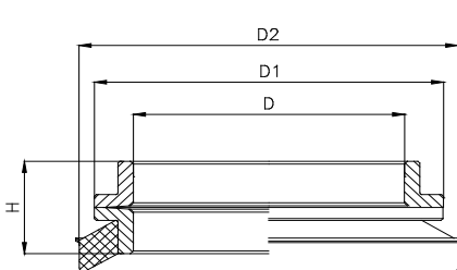
DD-CROSS-SECTION
